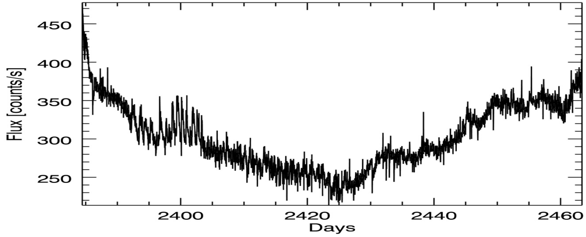
K2 Everest Light Curve
