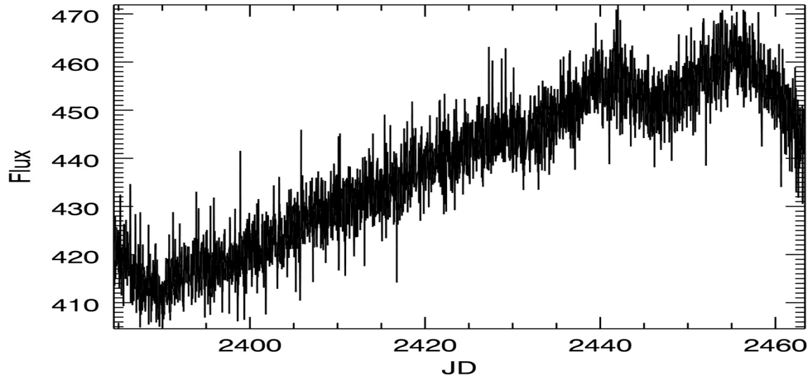
K2 Everest Light Curve
