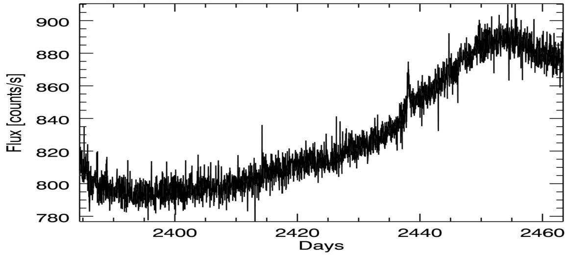
K2 Everest Light Curve
