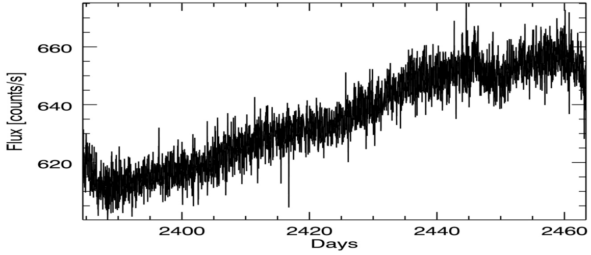
K2 Everest Light Curve
